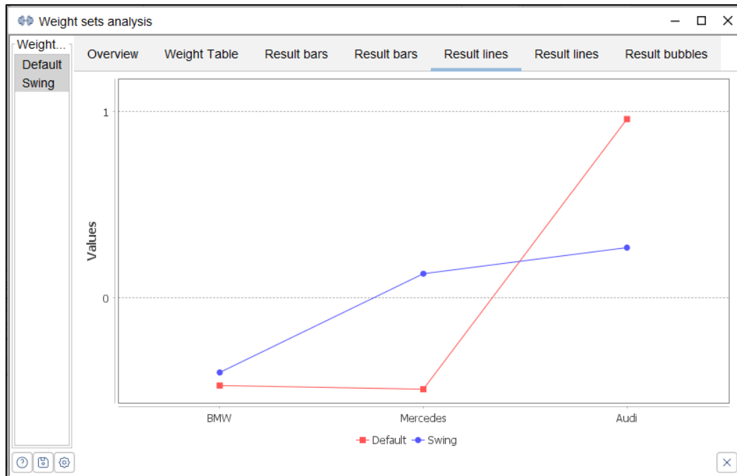
Figure 44. Weight sets analysis: result lines (1).
