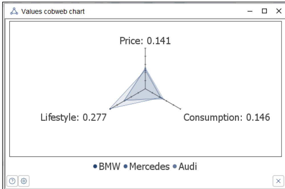
Figure 25: Cobweb chart of values
