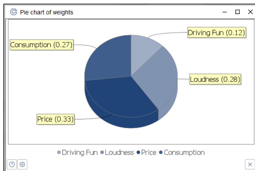
Figure 31: Pie chart of weights
