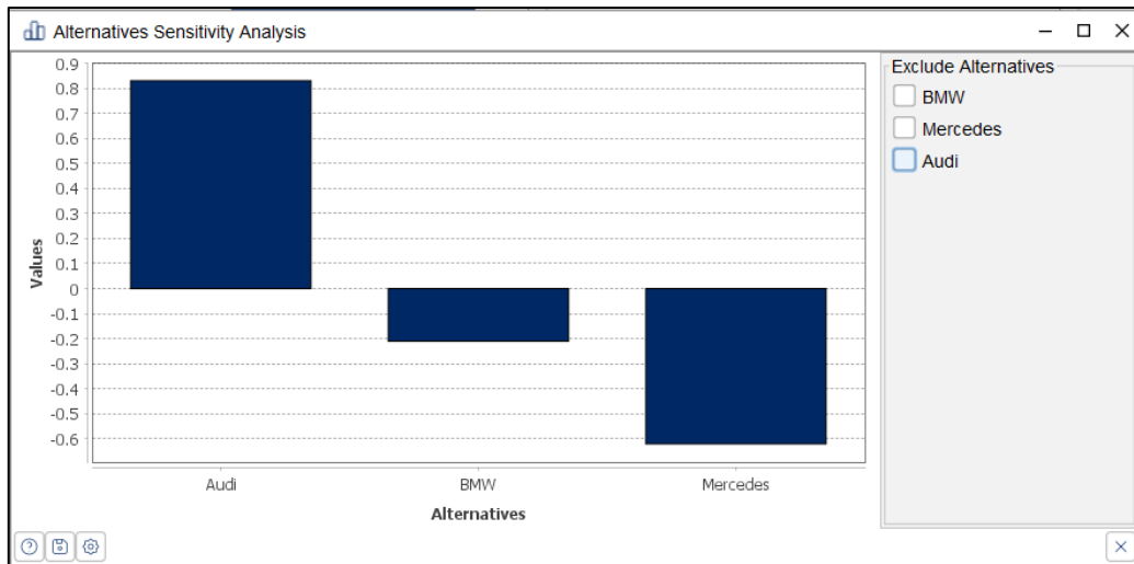
Figure 49: Sensitivity analysis for alternatives.
