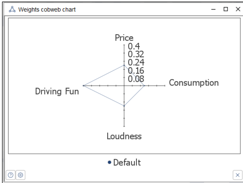
Figure 26: Cobweb chart of weights
