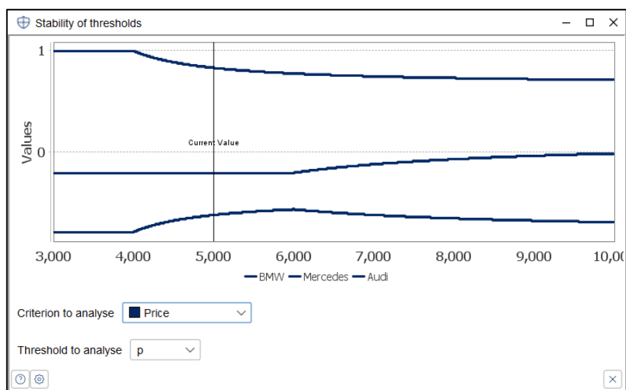
Figure 48: Sensitivity analysis for thresholds
