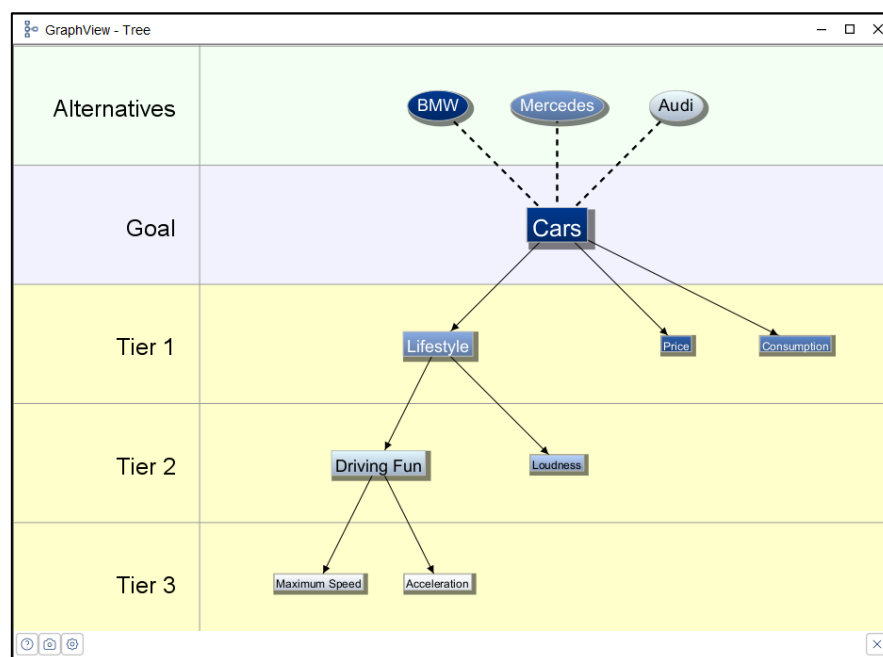
Figure 10: Graph View
