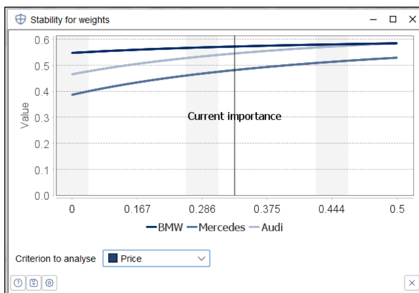
Figure 46: Sensitivity analysis for weights
