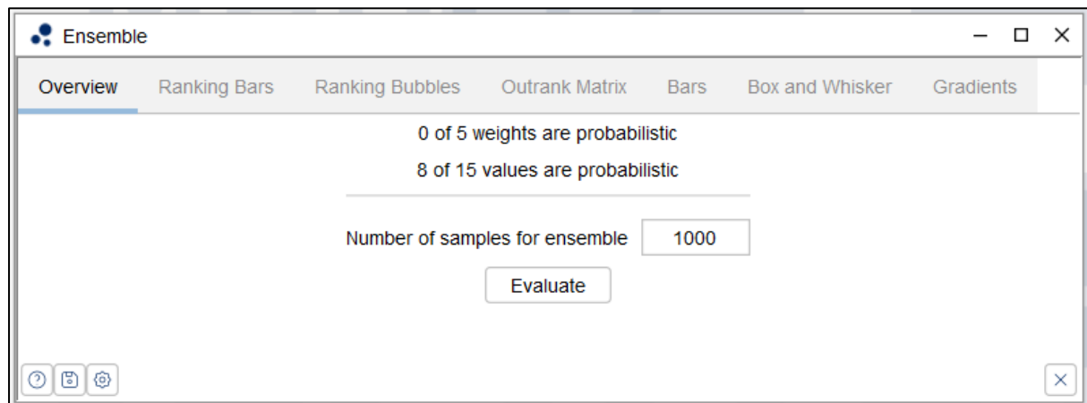
Figure 34: Ensemble
