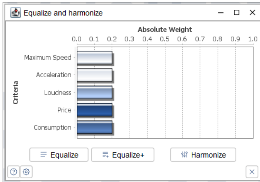
Figure 15: Equalize weights
