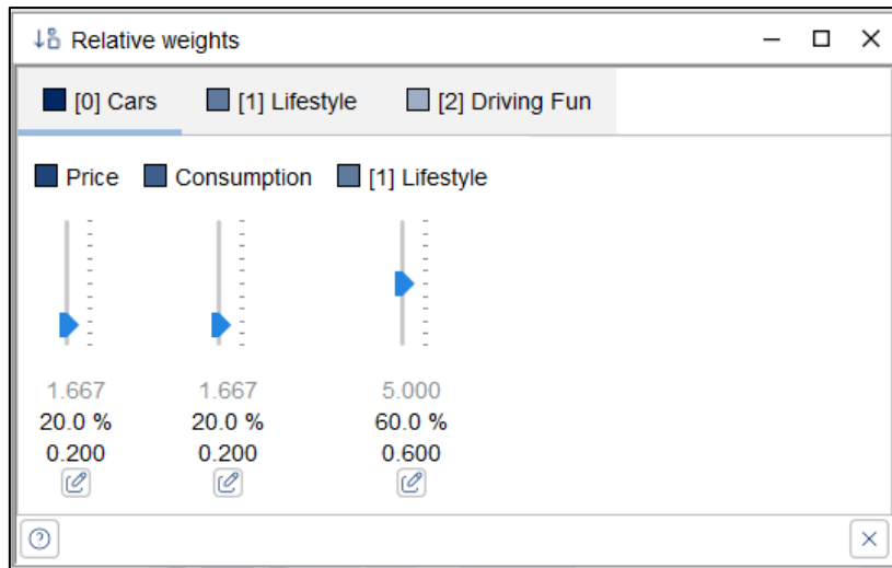
Figure 14: Direct Weights
