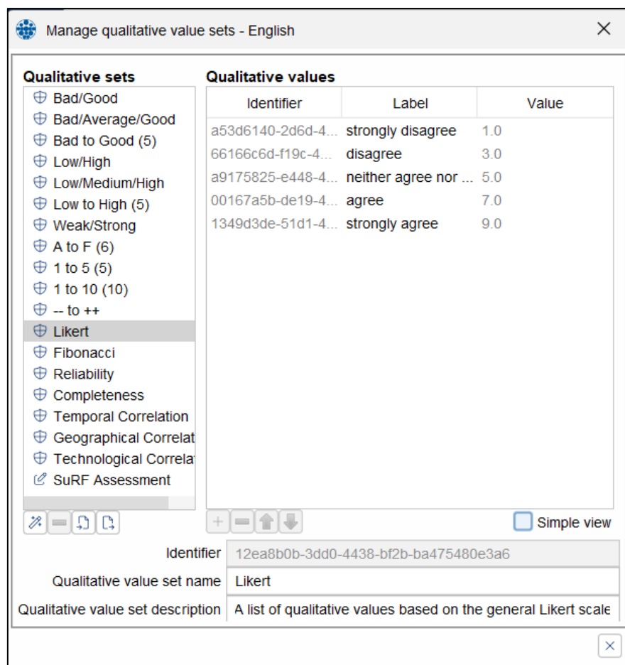
Figure 21: Qualitative sets
