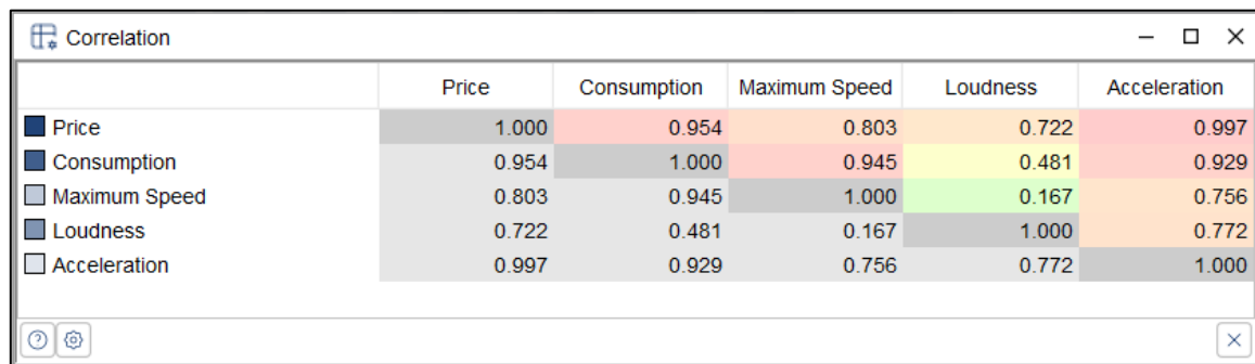
Figure 32: Correlation
