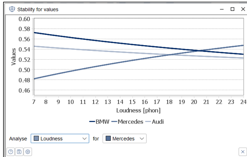
Figure 47: Sensitivity analysis for values
