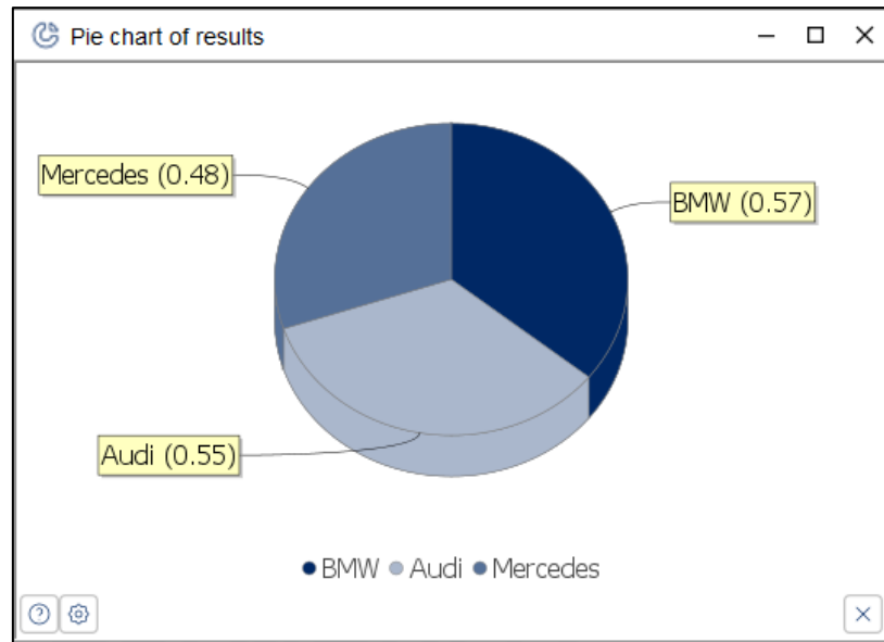
Figure 29: Pie chart of results
