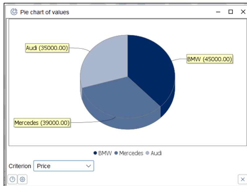
Figure 30: Pie chart of values
