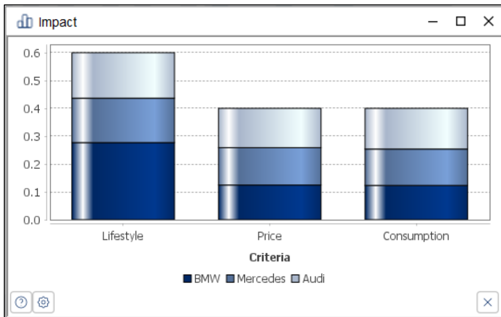
Figure 35: Impact
