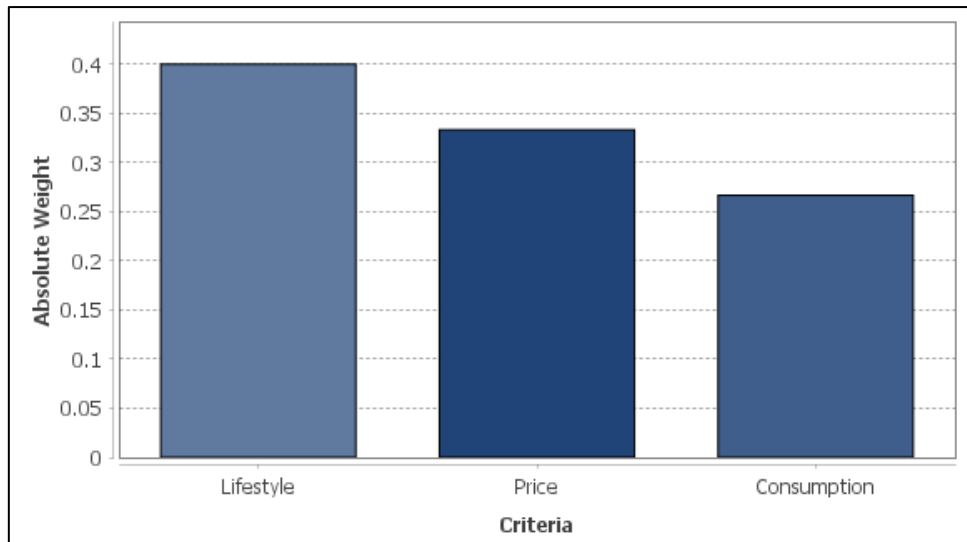
Figure 24: Bar chart of weights
