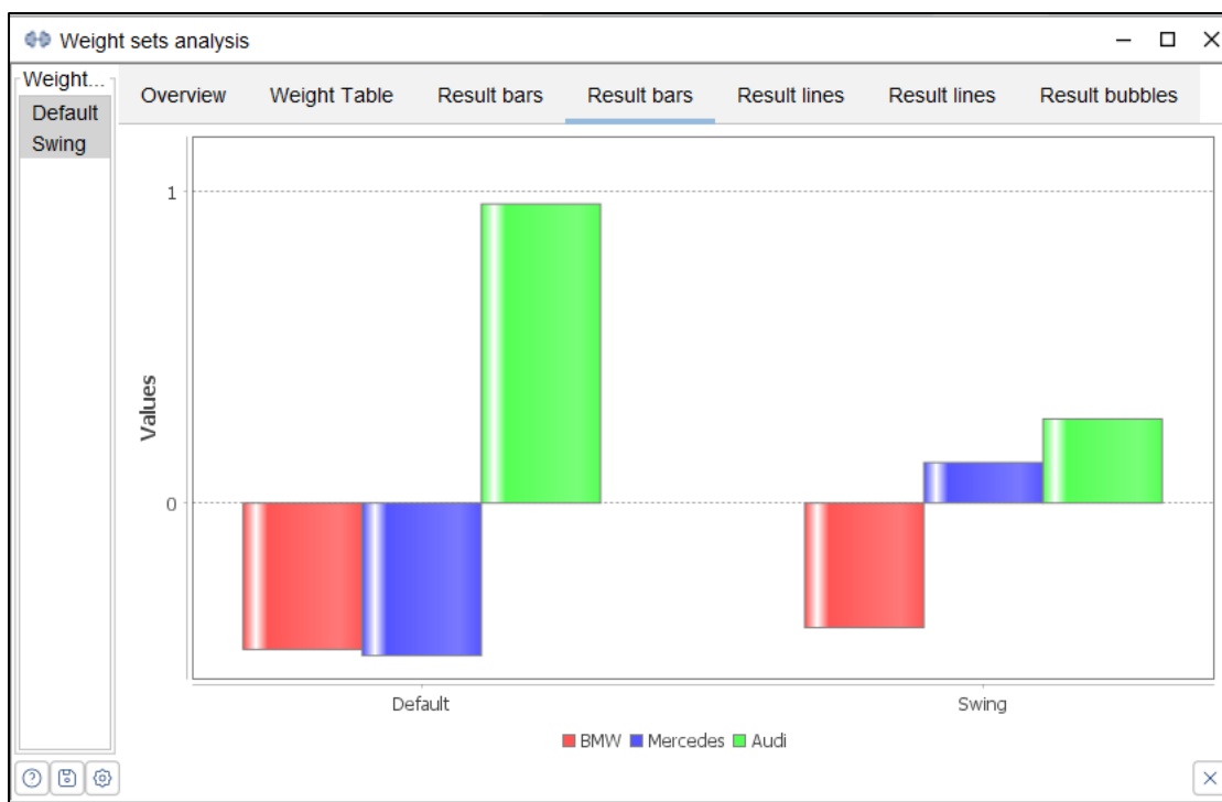
Figure 43. eight sets analysis: result bars (2).
