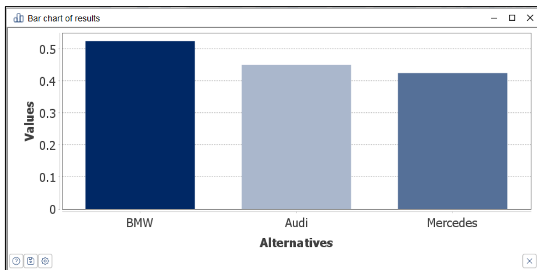
Figure 23: Bar chart of results
