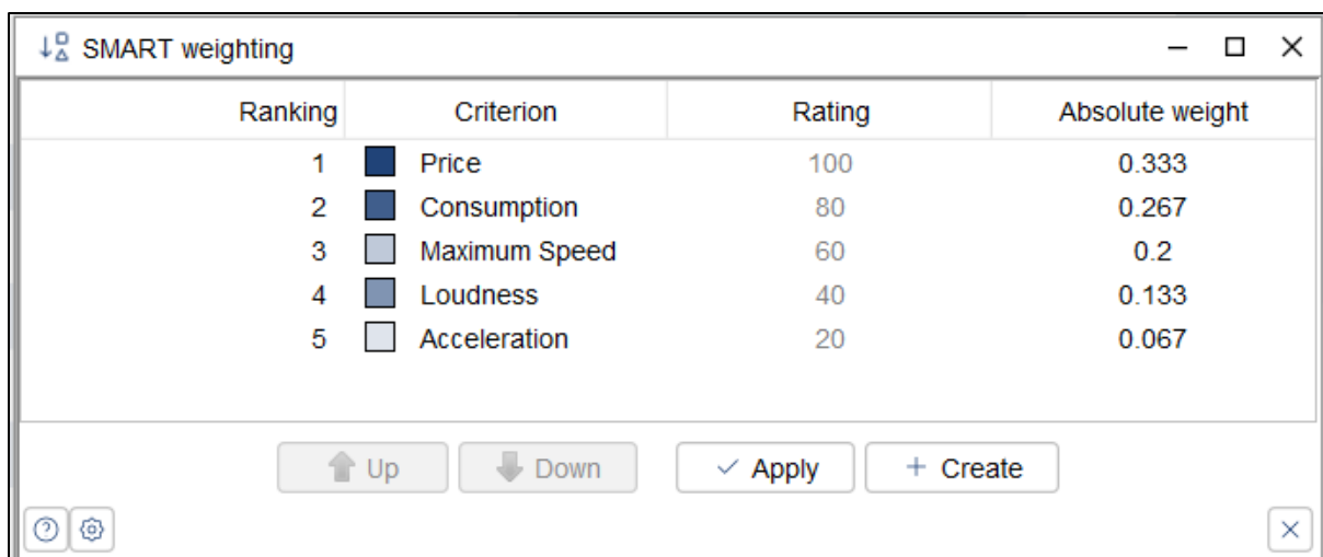
Figure 17: SMART weighting
