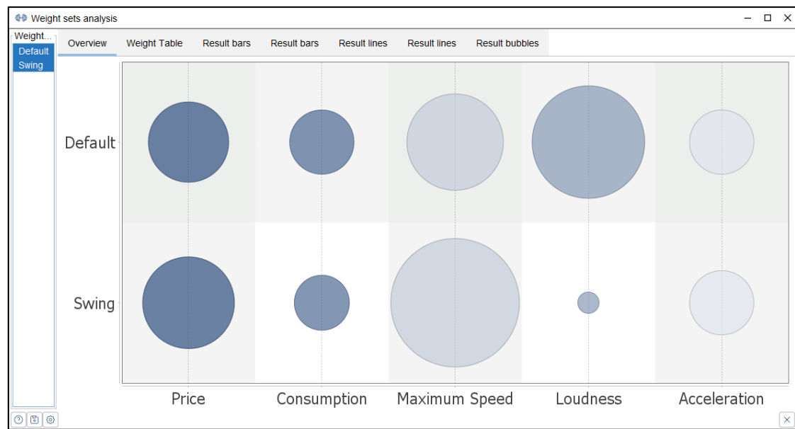
Figure 40: Weight sets analysis: overview.
