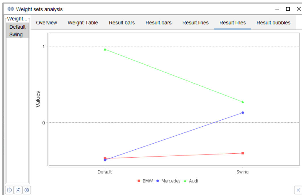
Figure 45. Weight sets analysis: result lines (2).
