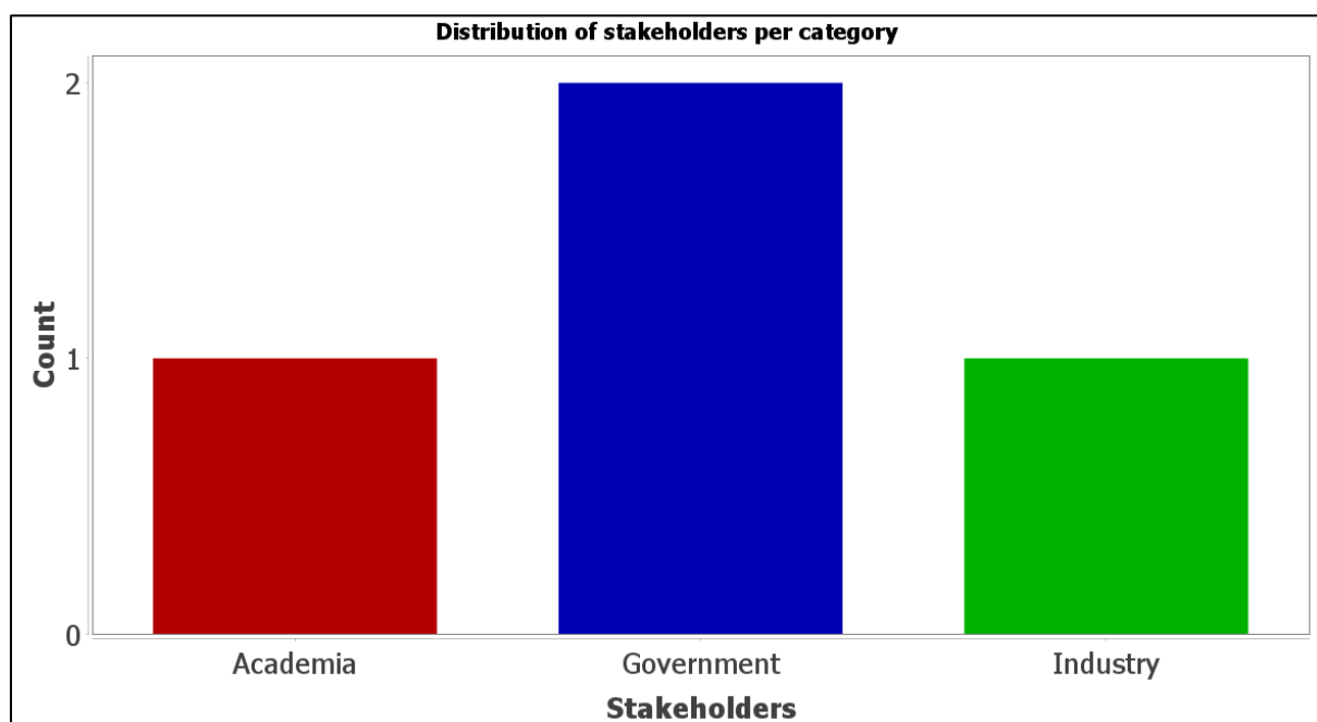
Figure 56: Statistics for weights tab of Plugin for online surveys – Running survey
