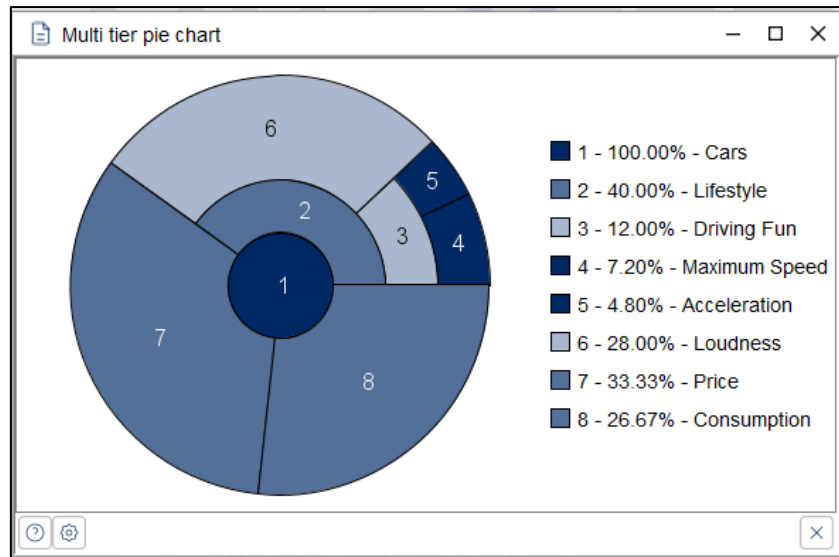
Figure 28: Multi-tier pie chart
