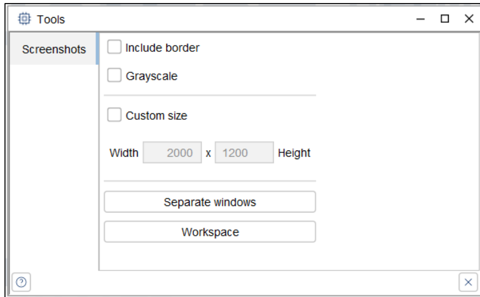
Figure 22: Tools
