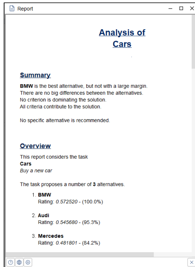
Figure 36: Report
