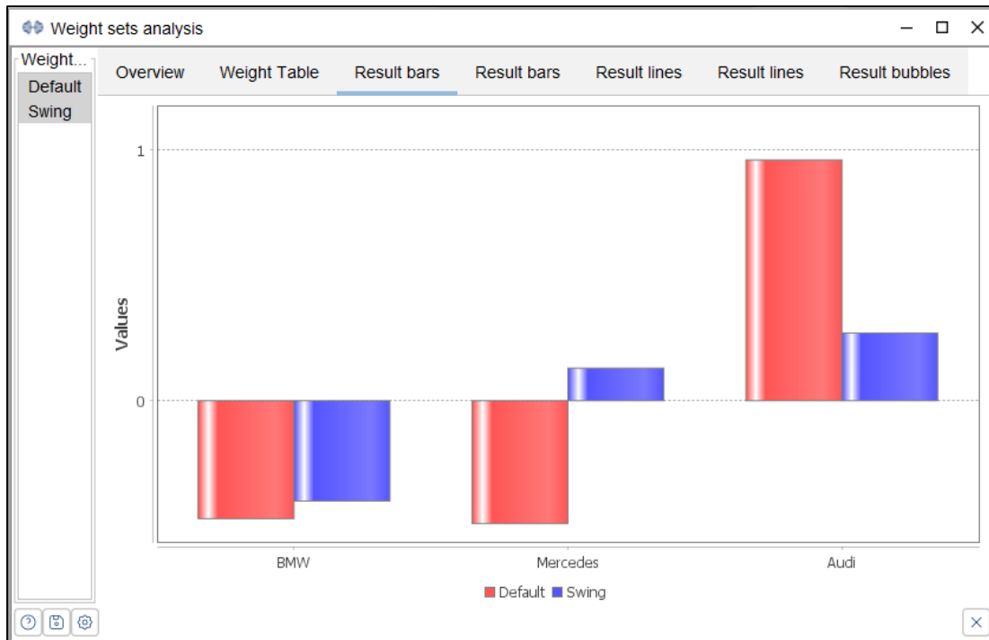
Figure 42. eight sets analysis: results bars (1).
